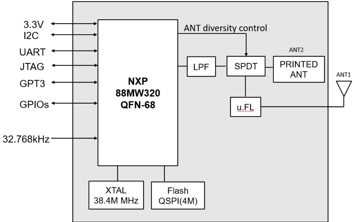
Block Diagram of AW-CU300A V3
